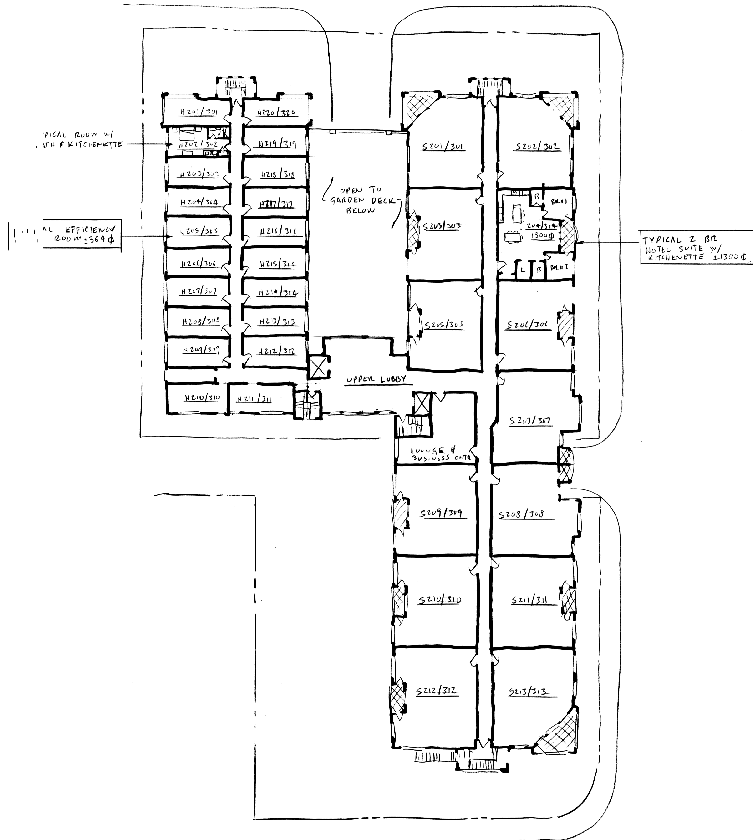
SECOND & THIRD FLOOR PLAN SCALE - 1" = 20'
